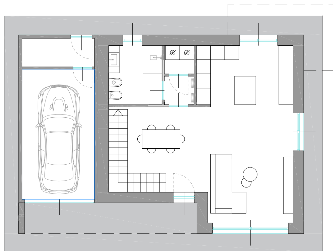
PIANO TERRA
