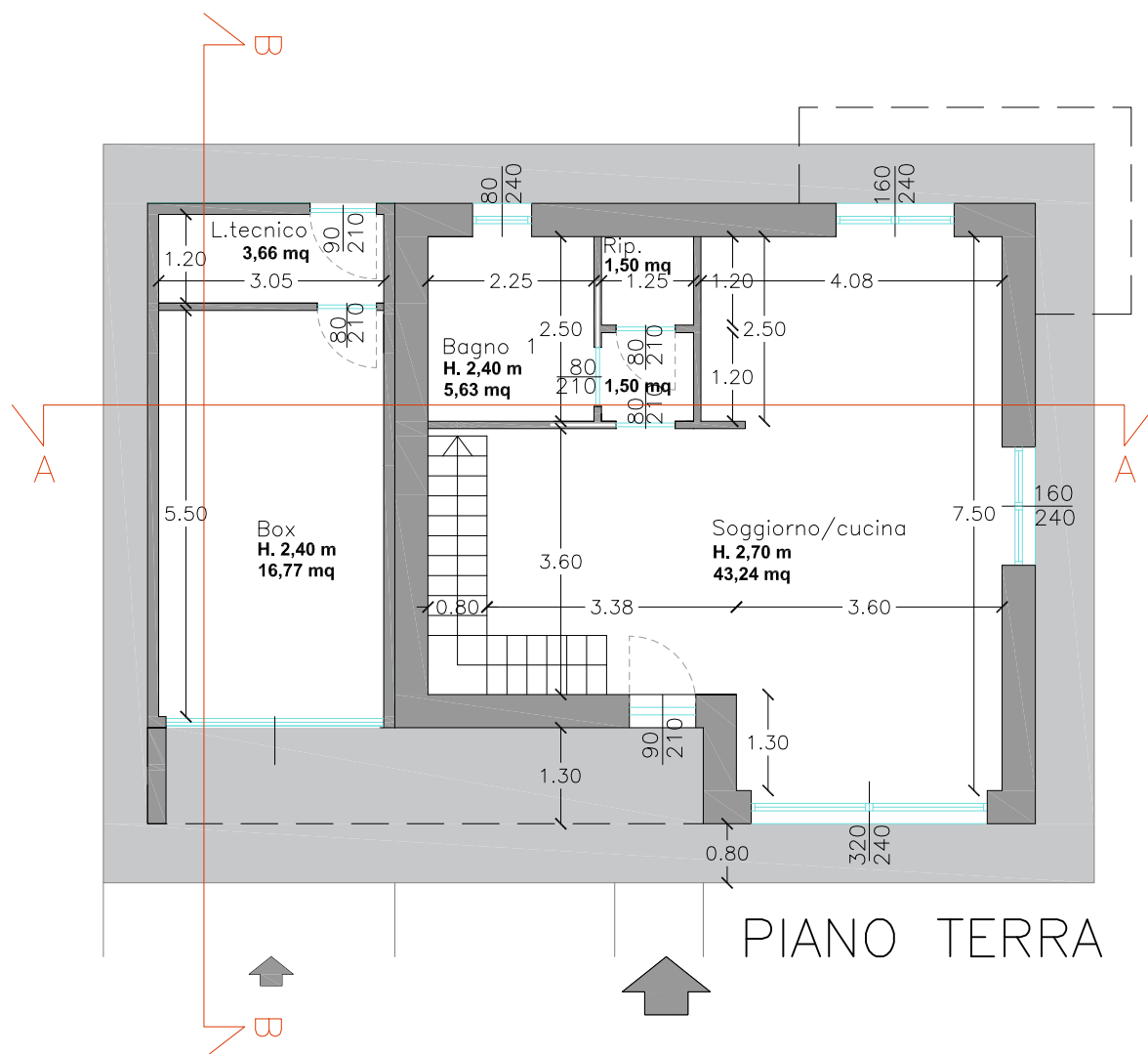
PIANO TERRA
